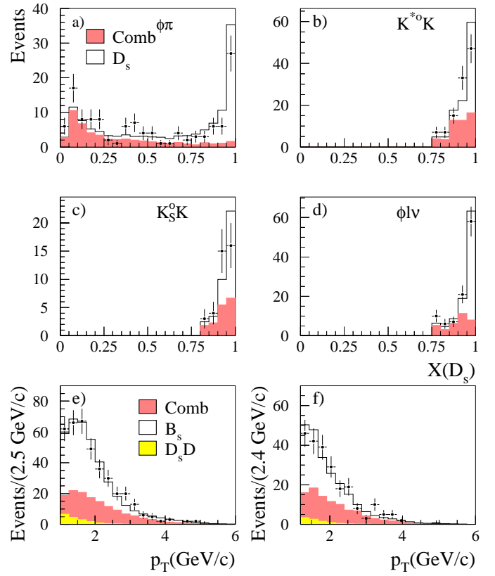
Fig. 5a–f. The plots illustrate the agreement between data and simulation for the variables used in the estimate of the B_s^0 purity on an event by event basis. a , b , c and d show the X_{D_s} distributions for the channels \phi\pi , \bar{K}^{*0}K , K_S^0K and \phi\ell^+ respectively. White histograms and shaded histograms represent the signal and the background respectively. e and f show the p_T distributions for the samples selected with p_T > 1 \text{ GeV}/c ( \phi\pi^+ and \phi\ell^+\nu ) and p_T > 1.2 \text{ GeV}/c (all the others) respectively. For the p_T distribution the D_s\bar{D} and the combinatorial background are considered separately
