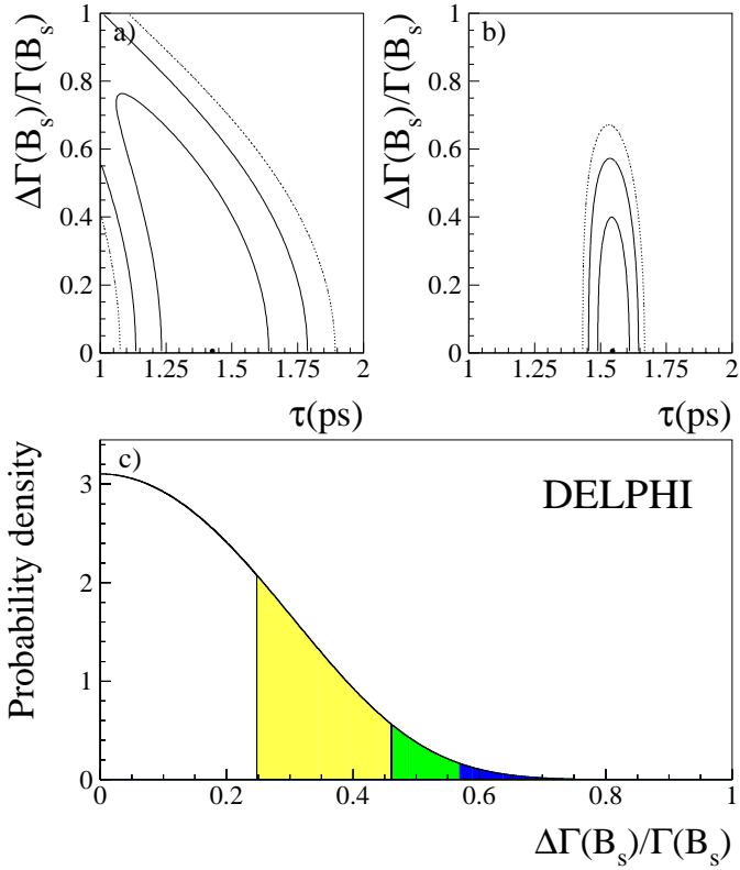
Fig. 10. a 68%, 95% and 99% C.L. contours of the negative log-likelihood in the plane \tau ( \equiv 1/\Gamma_{B_s} )- \Delta\Gamma_{B_s^0}/\Gamma_{B_s^0} evaluated on the D_s\ell sample. b Same as a but with the constraint \tau = \tau_{B_d^0} . c Probability density distribution for \Delta\Gamma_{B_s^0}/\Gamma_{B_s^0} ; the three shaded regions show the limits at 68 %, 95% and 99% C.L. respectively
