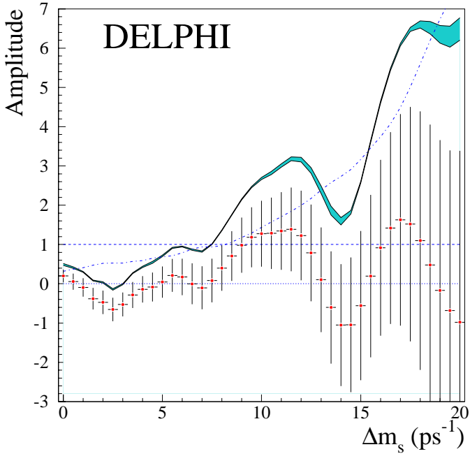
Fig. 13. Variation of the oscillation amplitude A as a function of \Delta m_s . The lower continuous line corresponds to A + 1.645 \sigma_A where \sigma_A includes statistical uncertainties only, while the shaded area includes the contribution from systematics. The dashed-dotted line corresponds to the sensitivity curve. The lines at A=0 and A=1 are also given
