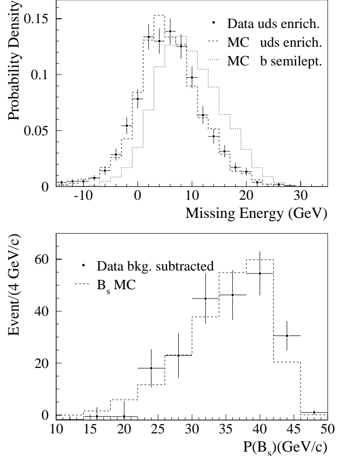
Fig. 6. The plot on the top shows the comparison between data and the simulation for the missing energy distribution after correction (see Sect. 3.6). The data (dots with error bars) and the simulation (dashed histogram) are enriched in light quark events. The dotted histogram shows the missing energy distribution in simulated b semileptonic decays. The plot on the bottom shows the comparison between the B_s^0 momentum distribution for simulated events and the one estimated from data in the signal region by subtracting the B_s^0 momentum distribution of events in the D_s side bands from that of the events in the signal region
