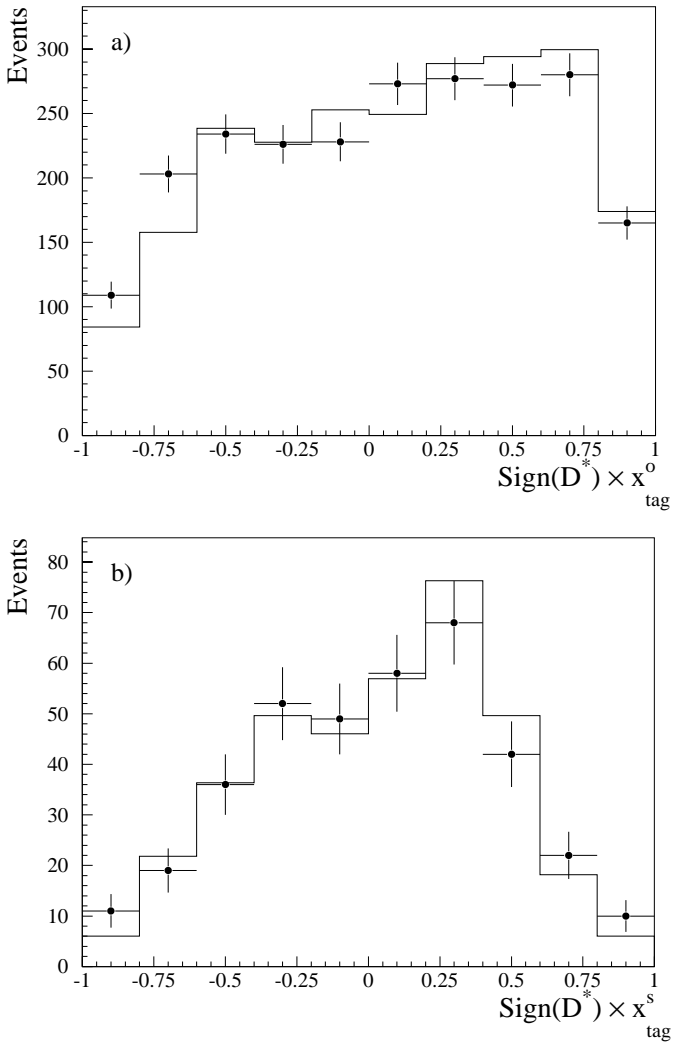
Fig. 11a,b. Check of the flavour tagging on the D^* sample. a Distribution of the product between the global tagging variable x_{tag}^o and the charge of the D^{*\pm} in the hemisphere opposite to the D^{*\pm} candidate. b Distribution of the product between the global tagging variable x_{tag}^s and the charge of the D^{*\pm} in the same hemisphere as the D^{*\pm} -lepton candidate. The full dots with the error bars represent the data. The histogram is obtained in the simulation. The non perfect separation is due to the mistag fraction of x_{tag} but also to the B_d^0 - \bar{B}_d^0 mixing
