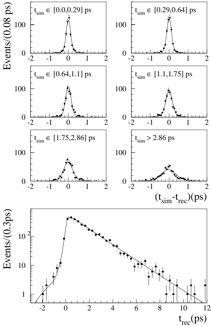
Fig. 7. The six plots on the top show the proper time resolution, defined as the difference between the generated time ( t_{sim} ) and the reconstructed time ( t_{rec} ), in bins of generated time on a sample of \phi\pi events simulated with the 94-95 Vertex Detector configuration. The plot on the bottom shows the distribution of the reconstructed time with the fit superimposed
