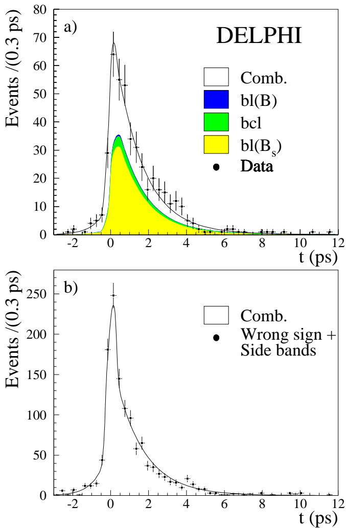
Fig. 8. D_s\ell sample. a Likelihood fit for events in the signal mass region. The points show the data and the curves correspond to the different contributions to the selected events. b The same as a but for “wrong-sign” events and for events situated in the side band region. The labels of the signal components refers to Sect. 3.5.1
