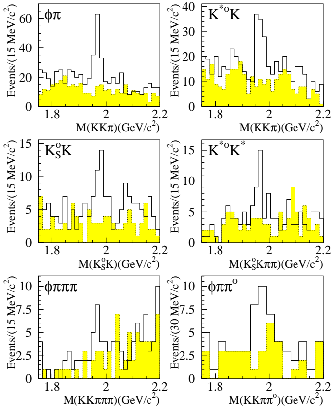
Fig. 2. Invariant mass distributions for D_s candidates in six non-leptonic decay modes ( \phi\pi^+ , \bar{K}^{*0}K^+ , K^0K^+ , \bar{K}^{*0}K^{*+} , \phi\pi^+\pi^-\pi^+ and \phi\pi^+\pi^0 ). The last three decay modes have been reconstructed using only the 94-95 statistics. The corresponding distribution for wrong-sign combinations are given by the shaded histograms
