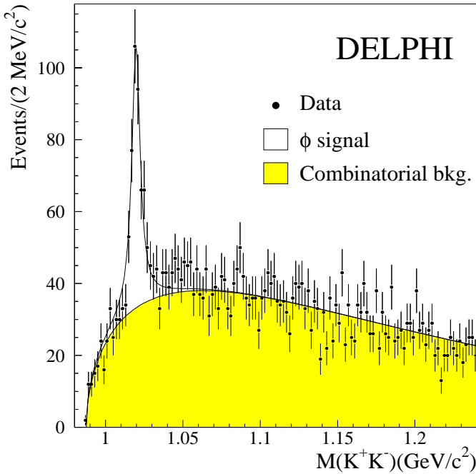
Fig. 4. K^+K^- invariant mass distribution of the \phi lh candidates. The curves show the result of the fit described in the text (the signal and the combinatorial background components are represented by the white and shaded histograms respectively)
