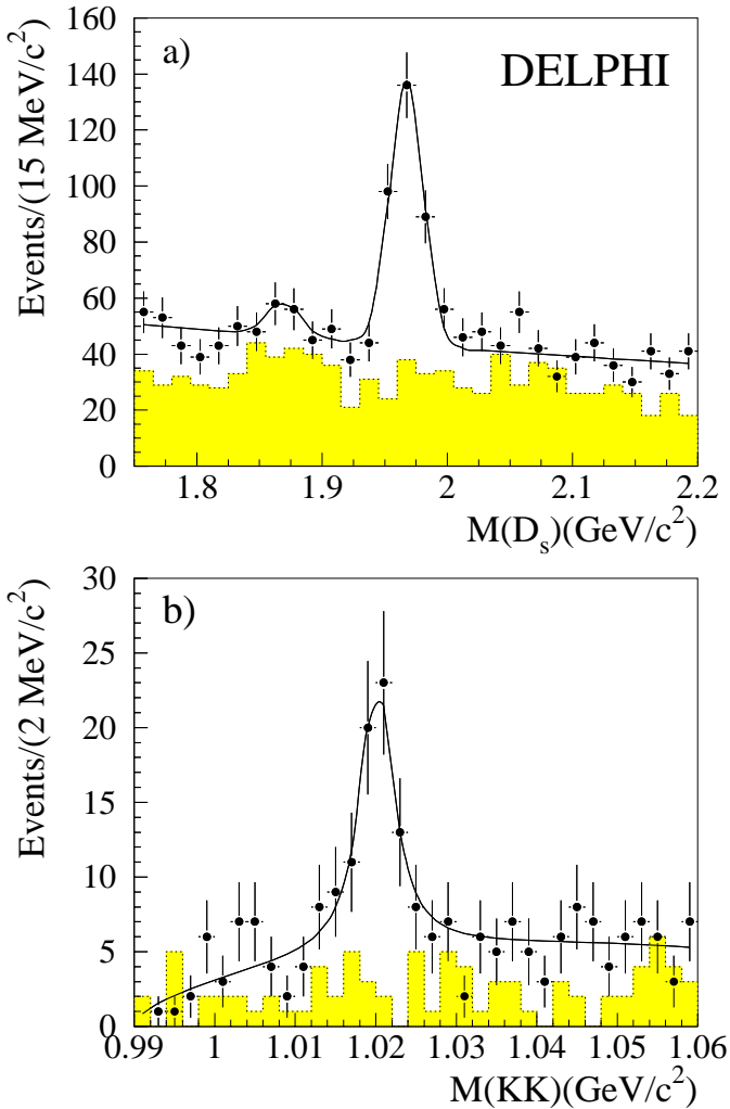
Fig. 3. a Invariant mass distributions for D_s candidates in non-leptonic decay modes ( \phi\pi^+ , \bar{K}^{*0}K^+ , K^0K^+ , \bar{K}^{*0}K^{*+} , \phi\pi^+\pi^-\pi^+ and \phi\pi^+\pi^0 ). b K^+K^- invariant mass distribution for D_s candidates selected in the two semileptonic decay modes. The corresponding distribution for wrong-sign combinations are given by the shaded histograms. The curves show the result of fits described in the text
