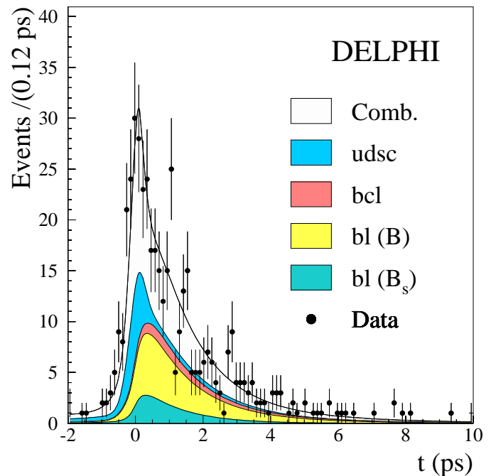
Fig. 9. \phi l h sample. Likelihood fit for events in the signal mass region. The points show the data and the curves correspond to the different contributions to the selected events. The labels of the signal components refers to Sect. 3.5.2
