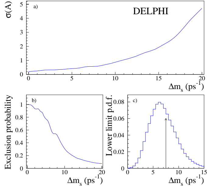
Fig. 15. a Variation of the error on the amplitude as a function of \Delta m_s . b Exclusion probability vs. \Delta m_s . c Lower limit probability density function vs. \Delta m_s
